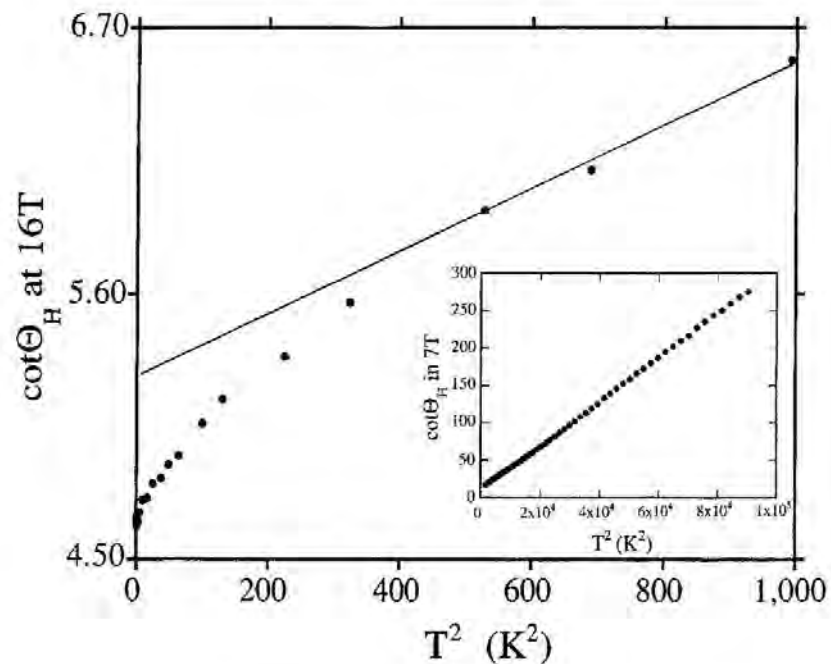
FIG. 8. The cotangent of the Hall angle plotted against T^2 below 30 K. The low-temperature data deviate significantly from the A + BT^2 dependence seen at high temperatures (inset), whose extrapolation is shown by the solid line.
