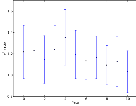
Figure 22: This is the ratio of \sigma^2 associated with the in-degree distribution of papers published in the same year for the data (years from 1992, 1993 etc. relabelled to 0, 1 etc.) divided by that of the modified model C (where the out-degree is determined by a lognormal distribution, above). The plot and error bars lie within 1.0 therefore the modified model C is consistent with the data. Therefore the modified model C is promising, a significant improvement on model A and B, figures 7 and 14, respectively. However, the data is always lower than the modified model C; the points are always above the 1.0 line and not as close to 1.0 as the model C which implies the need for modification of the parameters in model C. So modifying the out-degree does change the in-degree, which contradicts [18]. We conjecture that by changing the attention span parameter this model's \sigma^2 plot could increase to match the data.
