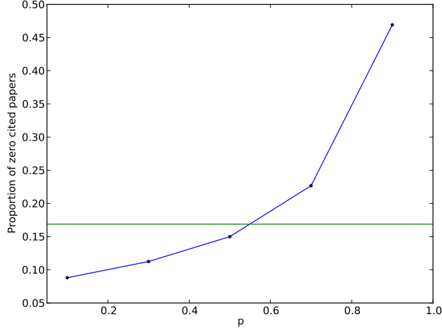
Figure 5: The blue line is a plot of the proportion of zero cited papers, z , in model A for a given probability of cumulative advantage p , against varying p . As expected, as p decreases uniform random attaching increases, this gives more opportunity for zero cited papers to attach. The green horizontal line is a constant line where the z is 0.169, the proportion of zero cited papers in the hep-th arXiv data set. Where the lines cross is where the proportion of zero cited papers in model A is equal to that of the data. This occurs at the desired p , 0.55.
