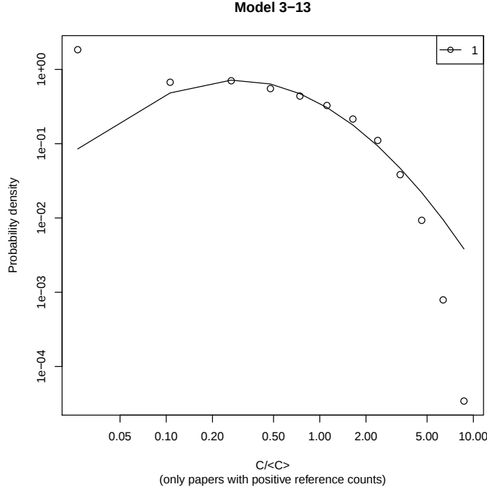
Figure 13: This is the overall in-degree distribution of probability density against normalised citation count for model B with best parameters p = 0.80 and \tau = 2000 papers. This \sigma^2 of this distribution is 1.05 \pm 0.18 . Compared to model A, figure 6, model B has more papers with high citation counts (the mid part of the distribution) making the tail longer and therefore increasing \sigma^2 (although the distribution maximum only goes up to approximately 10 citations like model A, figure 6). However, compared to the data, figure 2, the tail of model B needs to be longer, it needs to have a non-zero probability of having a normalised citation count greater than 50.
