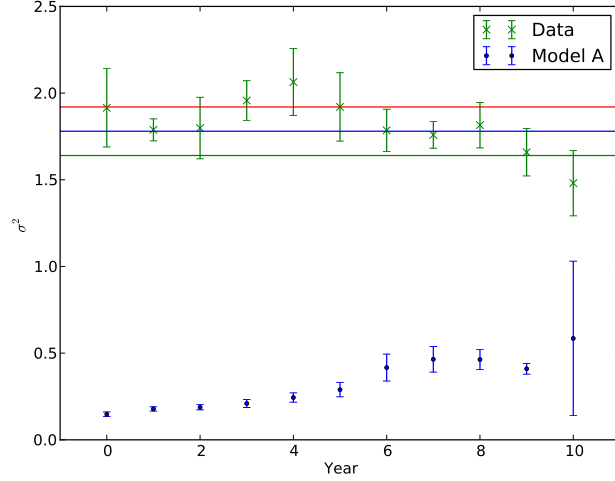
Figure 7: This is the \sigma^2 plot, the plot of \sigma^2 against year for both the data, in green, and model A, in blue. \sigma^2 is the width associated with the lognormal fitted to the in-degree distribution for papers published in the same year. On this plot the data's years from 1992 to 2002 are relabelled years 0 to 10 respectively. The data's average and one standard deviation are plotted as horizontal lines 1.78 \pm 0.14 . Model A and hep-th's \sigma^2 values are very different.
