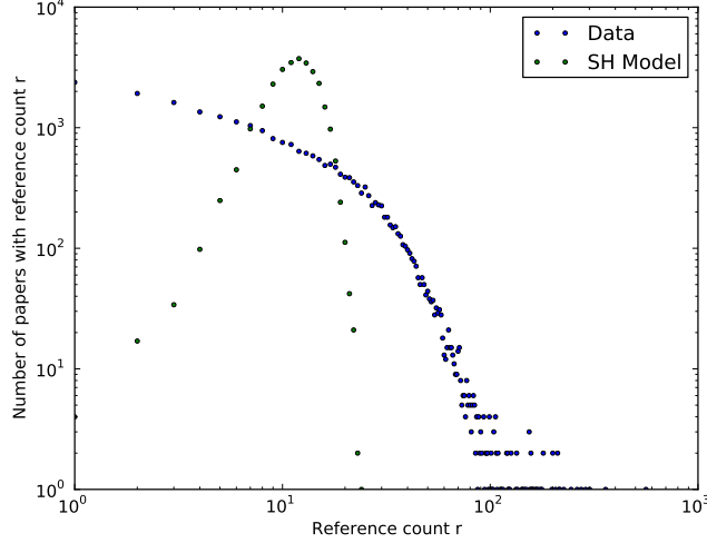
Figure 4: This is a plot of the out-degree distribution, number of papers with reference count r against reference count r , on a log-log plot for the data, in blue. Superimposed, in green, is a plot of the out-degree distribution used in our models, a normal distribution with the same mean 12.0 and standard deviation 3.0 as the whole hep-th data for the same number of publications, 27,000. This normal distribution used in our models is clearly not a good fit for the out-degree distribution found in the actual data.
