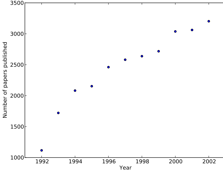
Figure 1: This is a graph of the number of papers published in a given year against year for the hep-th arXiv dataset. An increase is clear, the number of papers published per year increases in an approximately linear fashion, it is not constant. The number of publications released from 1992 to 2002 approximately triples from 1116 to 3203 papers. When year to year comparisons are made from the hep-th data to our citation network models, it is important to incorporate literature growth with year.
