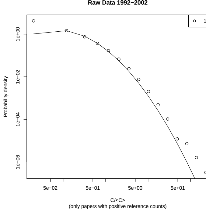
Figure 2: The citation distribution for all papers in the hep-th arXiv repository between 1992 and 2002. The points are the counts from logarithmic sized bins and plotted in terms of c/\langle c \rangle where \langle c \rangle is the average citation count taken over all papers. The line shows the form of the best fitting lognormal curve, equation (1) [9, 8]. The width of the distribution is \sigma^2 = 1.78 \pm 0.14 , large compared to the \sigma^2 \approx 1.3 found by [7, 17].
