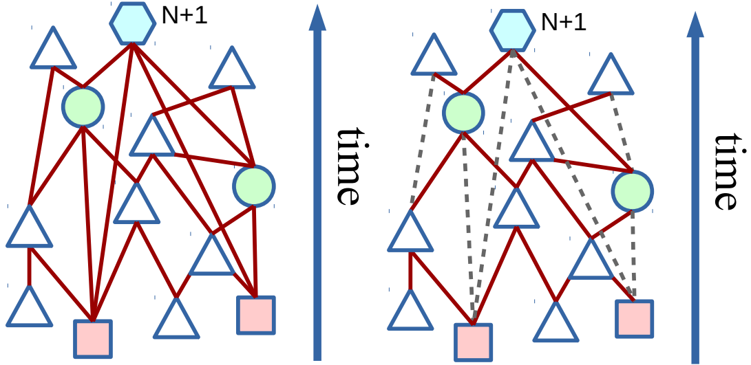
Figure 17: An illustration of the transitive reduction to identify citations to ‘core’ papers. On the left is the citation network of figure 15 after the new paper ( N + 1 ) (blue hexagon) and its references (green circles for its core references, red squares for its subsidiary references) have been added. On the right is the transitive reduction of this network where the dashed grey edges are the ones removed under transitive reduction. In this case, after transitive reduction the new paper ( N + 1 ) is only linked to the core papers in its references. The declustering method described in the text produces the same result in this case, but not in general.
