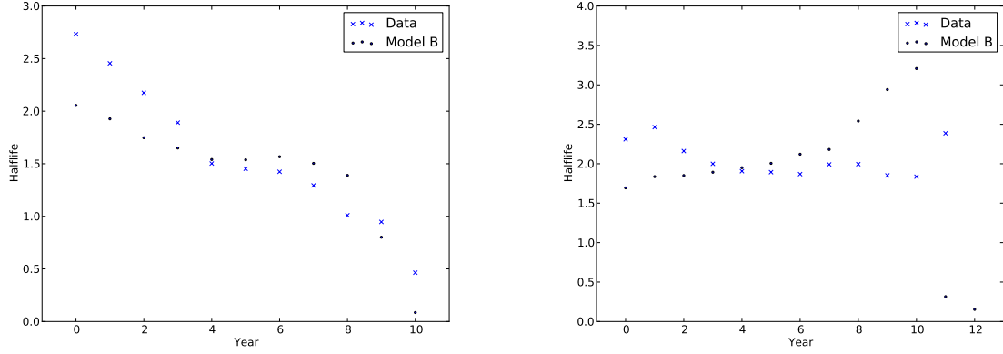
Figure 11: In figures we compare/contrast the measured half-life T_{1/2} for the hep-th data (crosses) and the output from model B using the best parameter values of p = 0.80 and \tau = 2000 (dots), for normal time (left) and rank time (right) in years. On the left we show half-lives measured from the the hep-th data, crosses, along with those derived from the output of model B, dots, (for p=0.80 , \tau = 2000 papers) against calendar year. On the left the same is shown but where rank time has been used.
