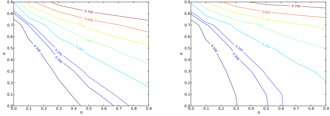
Figure 16: The fraction of zero cited papers found in the output from model C. The lines represent different fractions of zero cited papers z_c found for varying (p, q) values for a fixed attention span (defined below) of \tau = 200 papers on the left and \tau = 2000 papers on the right. The line of constant z_c equivalent to the hep-th data's z value, z_{\text{data}} = 0.169 . There are a family of (p, q) solutions ranging from (p, q) = (0.8, 0) to (p, q) = (0, 0.45) , one of the purple contour lines. Note that (p, q) = (0.8, 0) , is simply model B, i.e. there are no q steps only a mixture of cumulative advantage and uniform attachment with an overall time-decay factor. For the ‘unreasonable’ value of \tau = 2000 on the right, the solution of (p, q) = (0.0, 0.80) for z_{\text{modelC}} = z_{\text{data}} = 0.169 is the same as in contour for \tau = 200 papers. Along the q axis the solution for z_{\text{data}} = 0.169 when \tau = 2000 is (p, q) = (0, 0.51) , as opposed to (0, 0.66) for \tau = 200 . Although the attention span \tau has changed by a factor of 10, q has only changed by 0.15. For q < 0.3 this contour can be treated as approximately equivalent to that for \tau = 2000 papers. Therefore it is valid to just use one contour plot for \tau = 200 papers.
