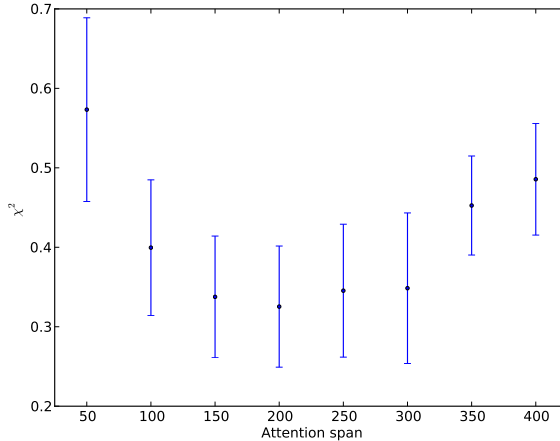
Figure 18: Plot of \chi^2 (the squared difference between the \sigma^2 of the data and the model C for fixed (p, q) = (0.55, 0.20) ) against varying attention span \tau measured in papers. Results show the mean and standard deviation for 10 runs of model C at each parameter value. The minimum is at 200 \pm 50 papers.
