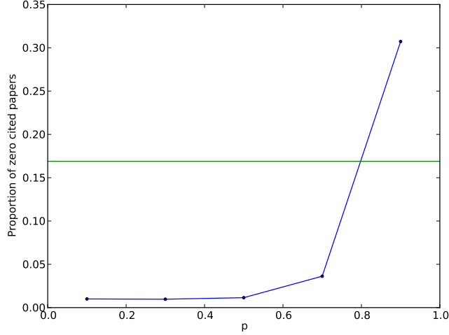
Figure 9: The blue data points show the z found for model B for a fixed \tau of 2000 papers and given probability of cumulative advantage p , against varying p . The green horizontal line gives the value for z found in the hep-th data, namely z = 0.169 . Interpolating from the model output suggests a value of around p = 0.80 is needed.
