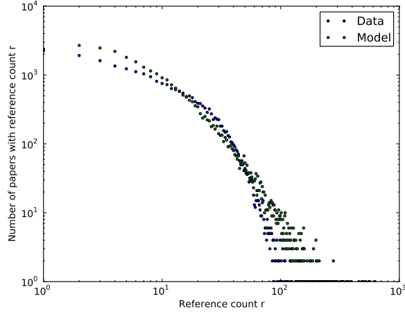
Figure 21: This is a plot of the out-degree distribution of 27,000 publications from the hep-th arXiv data, in blue, on a log-log plot. Superimposed, in green, is a plot of 27,000 numbers generated by the lognormal distribution fitted to the out-degree of the hep-th arXiv data. We observe that the lognormal is a better fit to the data than the normal in figure 4.
